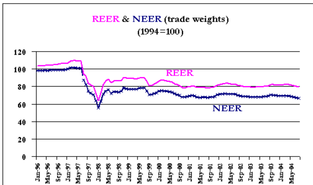
Figure 2: REER & NEER
